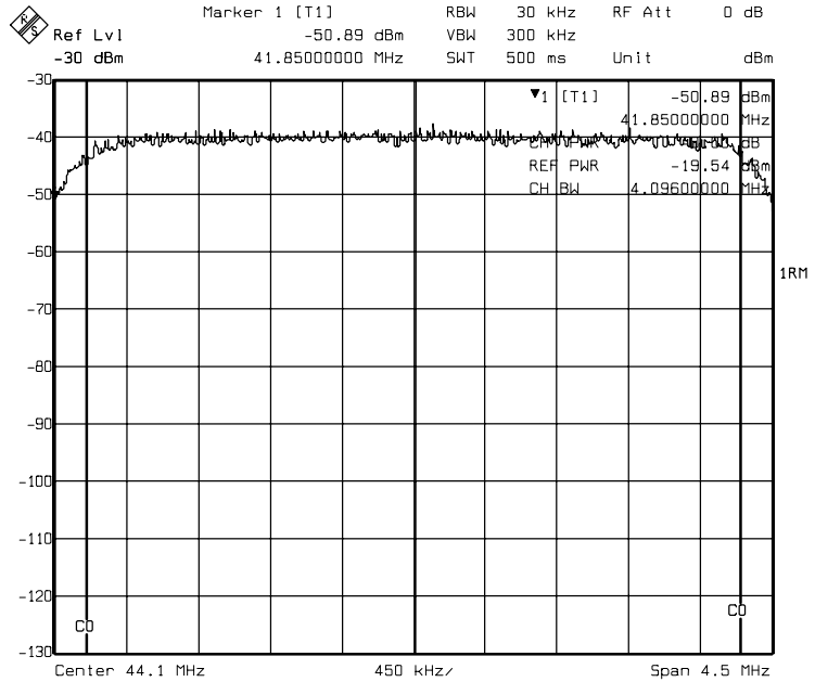
Fig. 5 Measurement of channel power in the transmit channel
