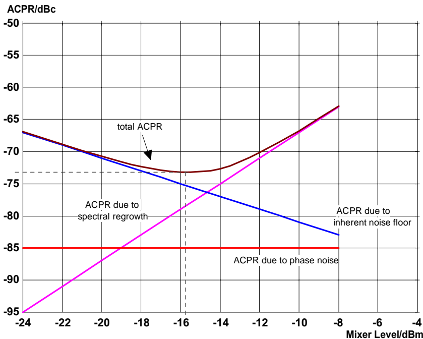
Fig. 2 Contributions for inherent ACPR of FSEA spectrum analyzer dependent on mixer level (= channel power at the input mixer)
