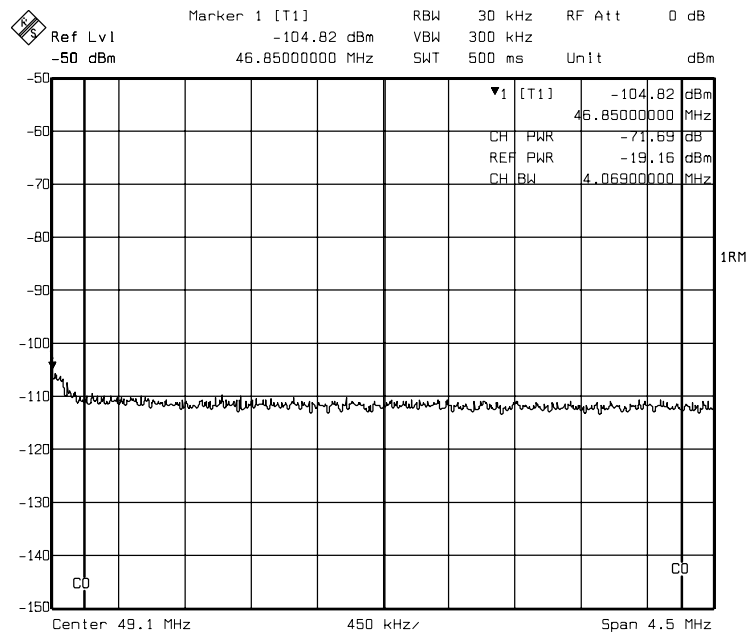
Fig. 6 Measurement of channel power in the upper adjacent channel
